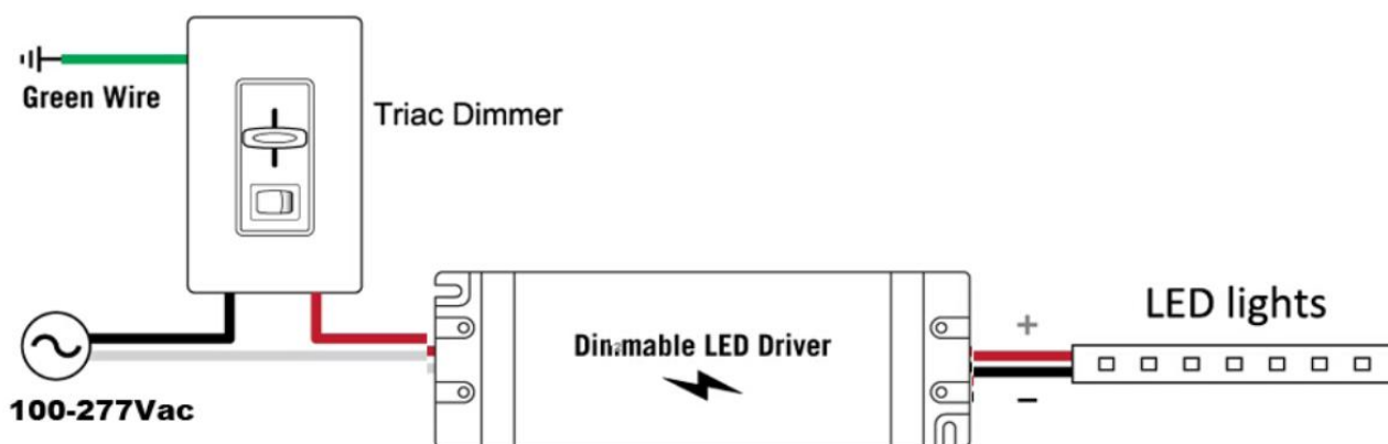
产品接线示意图/ Product Connection Diagram
